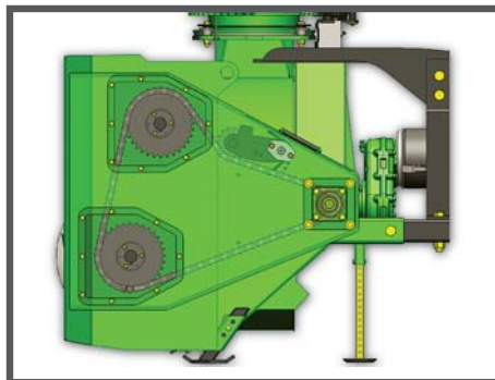
Drive chain, sprockets and tensioner shown in the enclosed chain case. The enclosed chain case eliminates snow build up on sprockets and chain extends life of the drive system.
