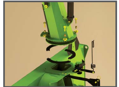
A high molecular UHMW bearing area keeps freeze ups to a minimum in the coldest weather conditions.
